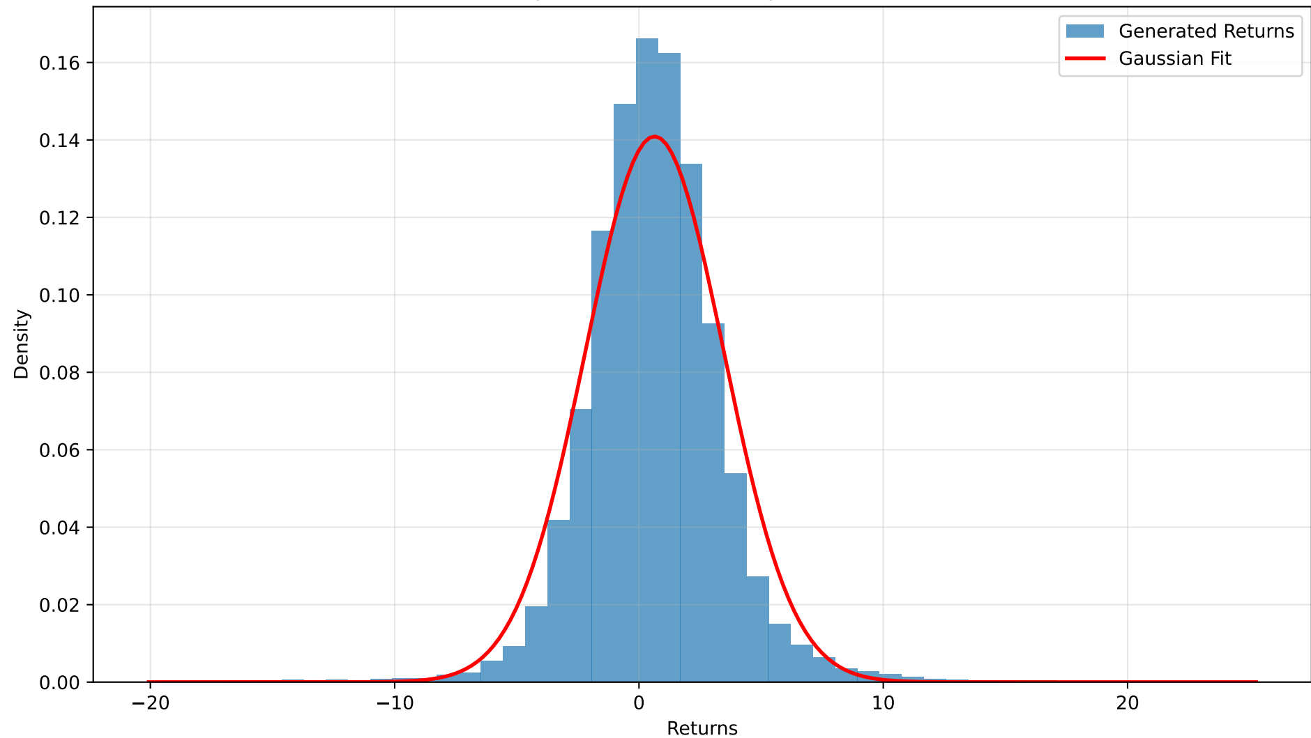
Explicit Conditioned: Stylized Facts
