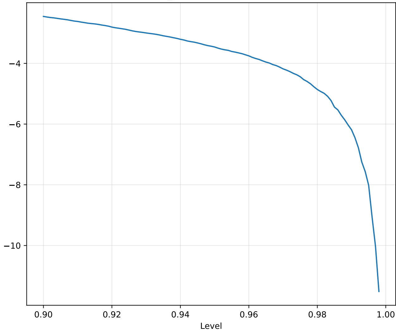
Explicit_Conditioned: VaR Curve
