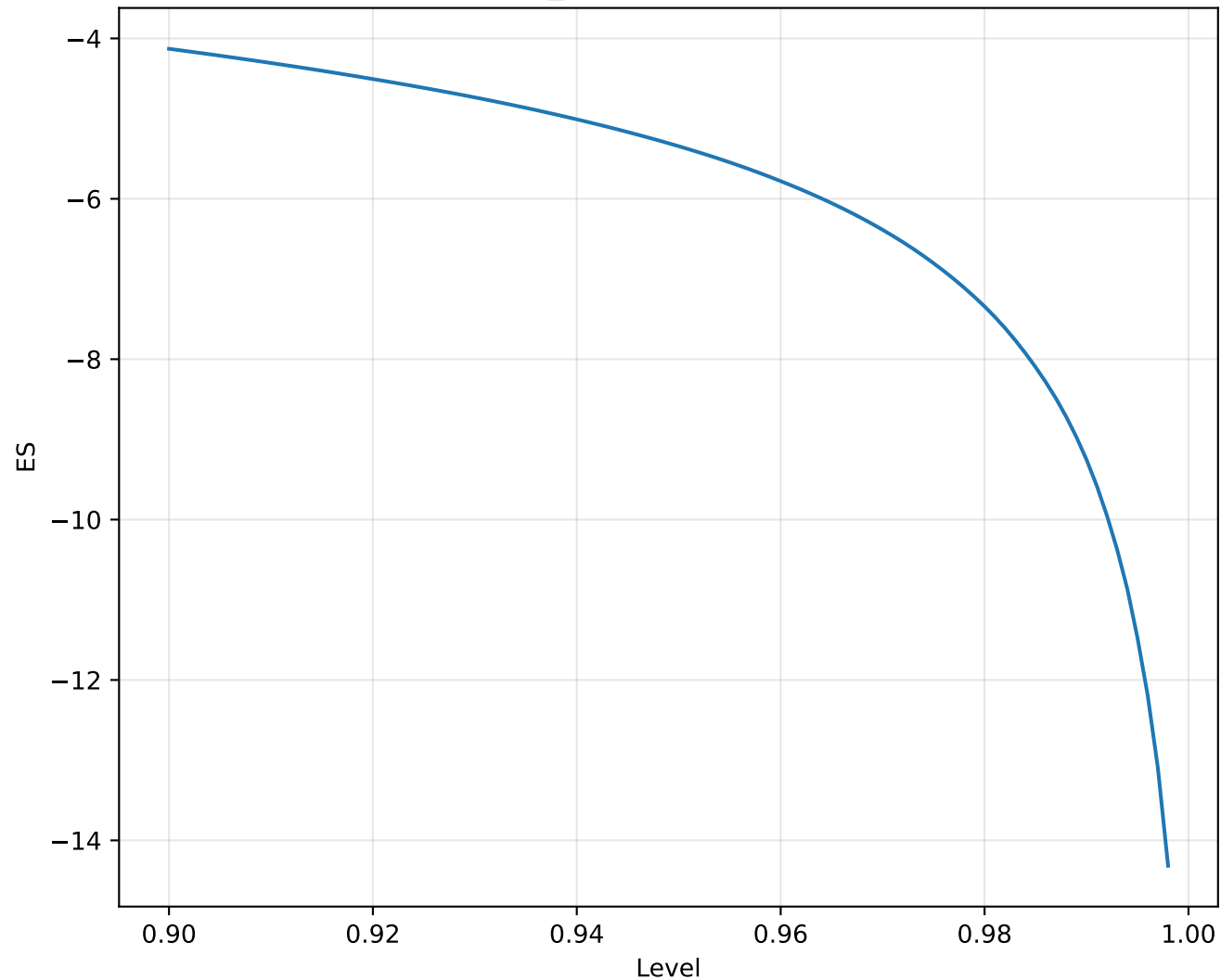
Explicit_Conditioned: ES Curve
