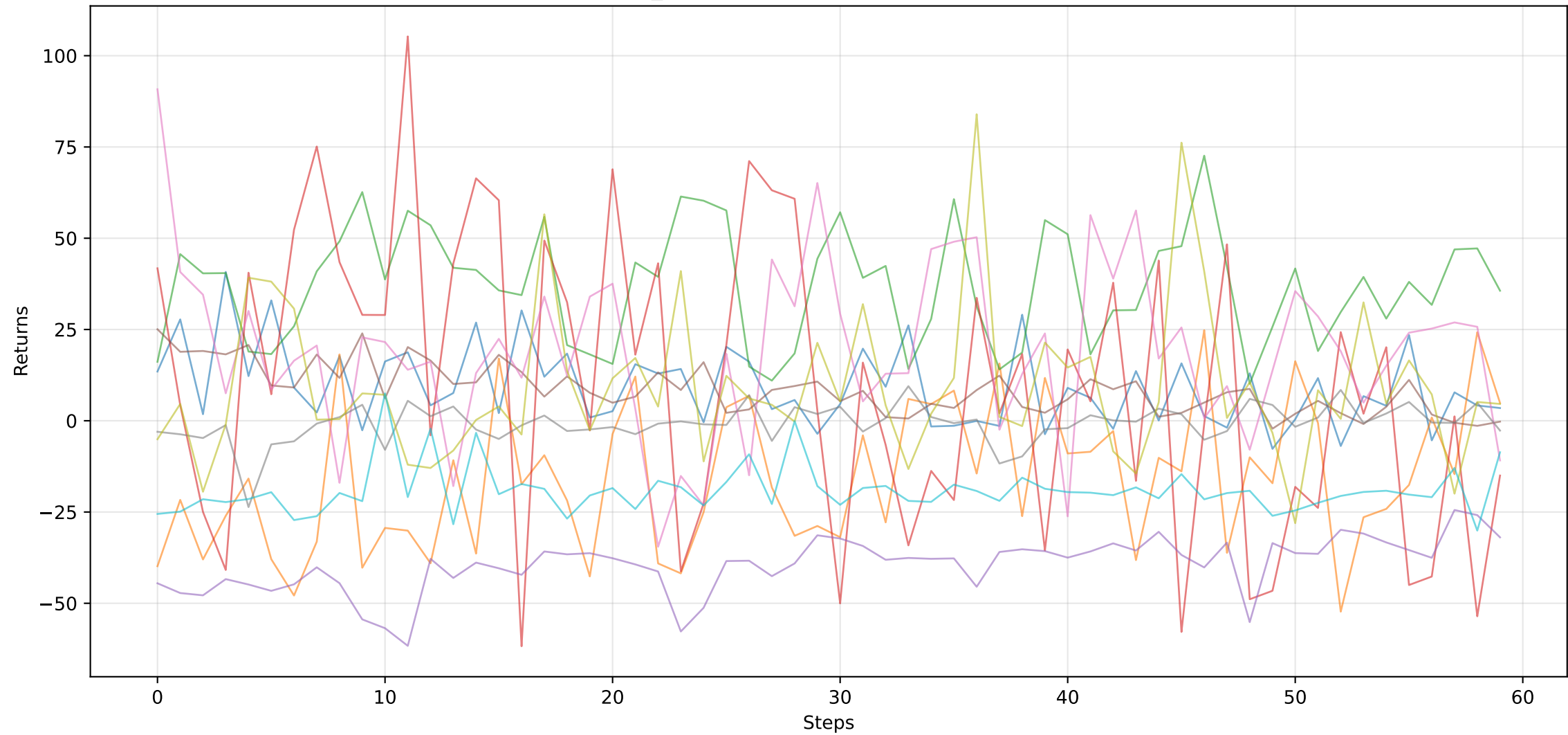
LLM_Conditioned: Sample Paths (n=10)
