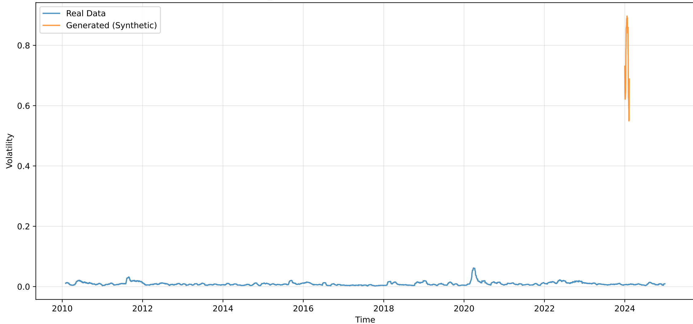
Zero_Conditioned: Rolling Volatility (window=20)
