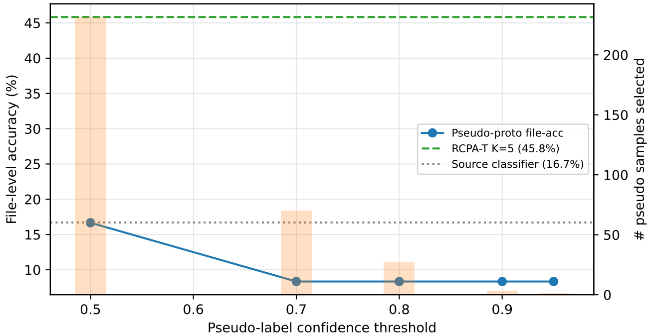
Pseudo-proto TTA threshold sweep (RX1→RX2, cal Block A only)
