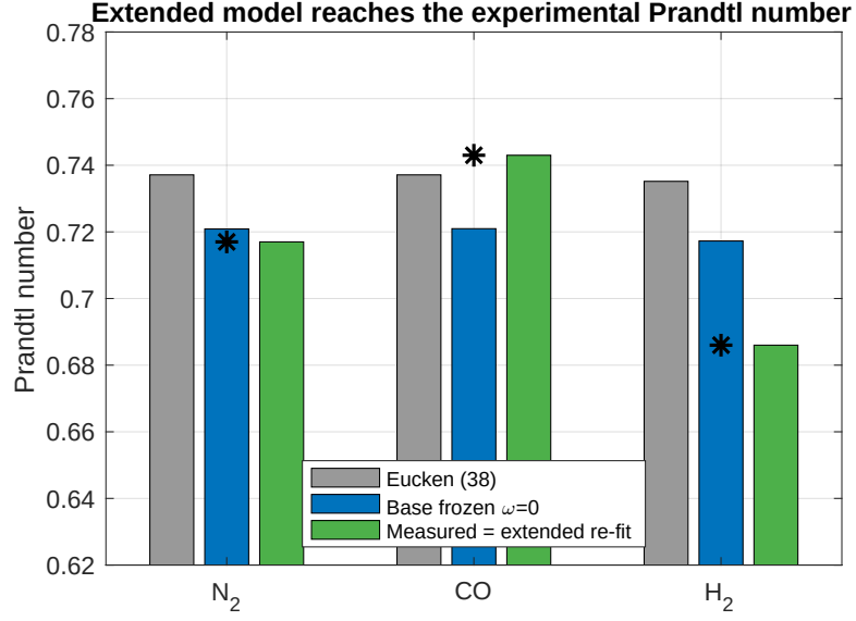
Figure 3: Per-gas Prandtl number: Eucken value, base-frozen value ( \omega = 0 ), and the measured value, which the re-fitted extended model reaches exactly.
