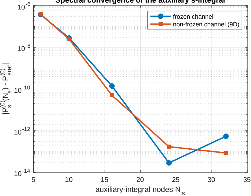
Spectral convergence of the auxiliary s-integral
