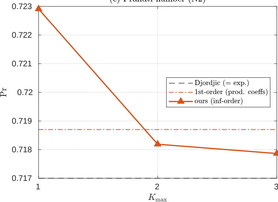
(c) Prandtl number (N2)
