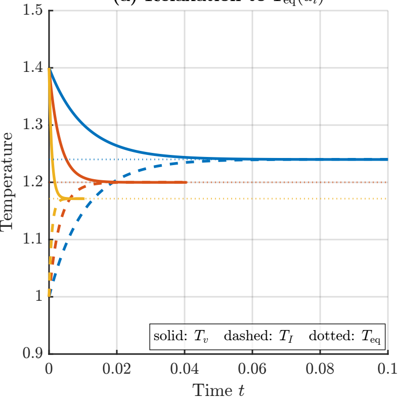
(a) Relaxation to T_{\text{eq}}(d_i)
