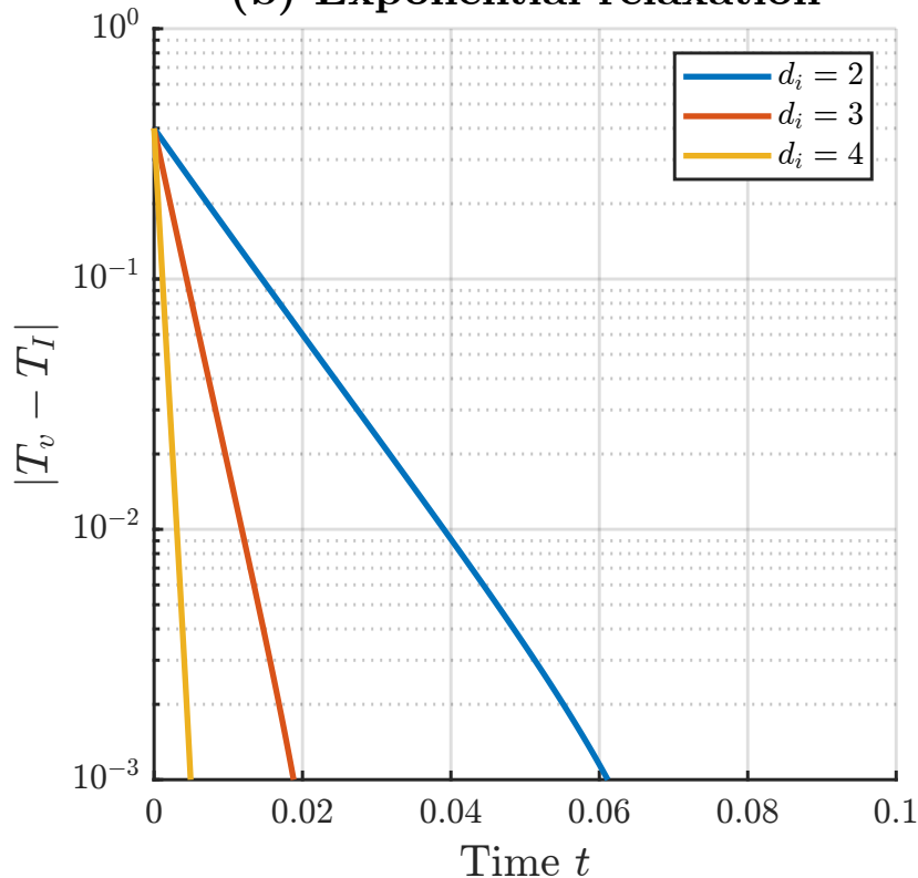
(b) Exponential relaxation
