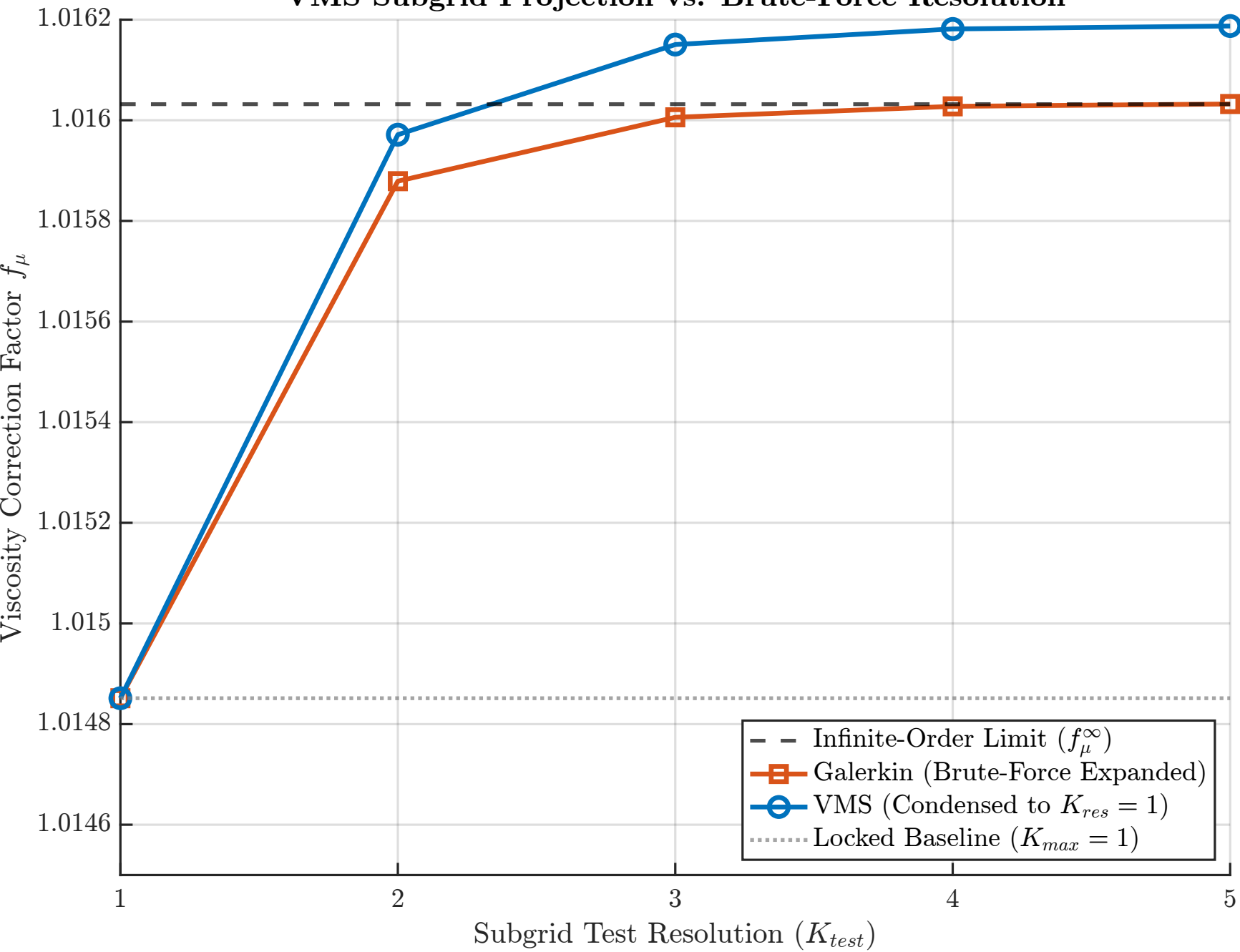
VMS Subgrid Projection vs. Brute-Force Resolution
