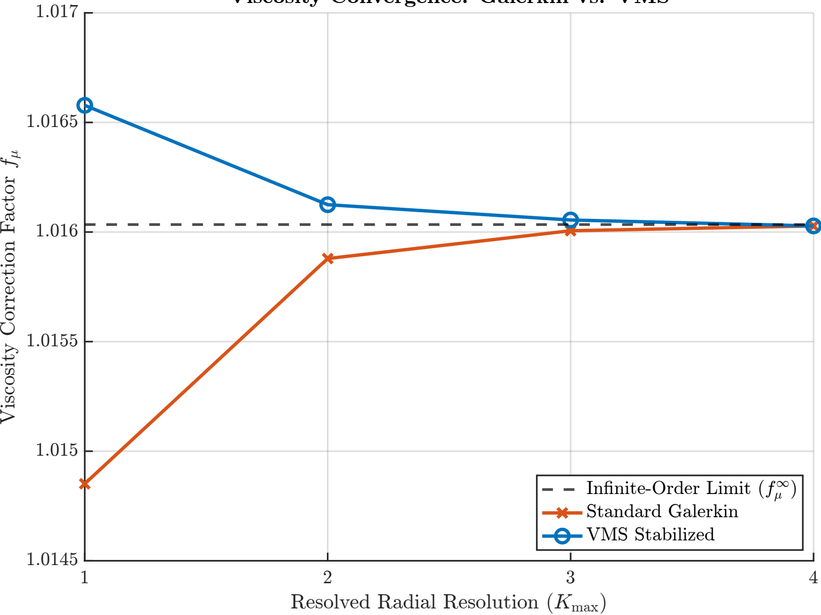
Viscosity Convergence: Galerkin vs. VMS
