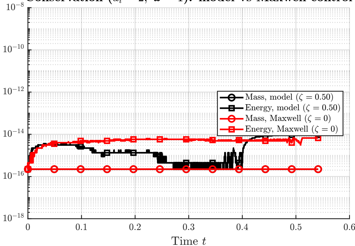
Conservation ( d_i = 2, \omega = 1 ): model vs Maxwell control
