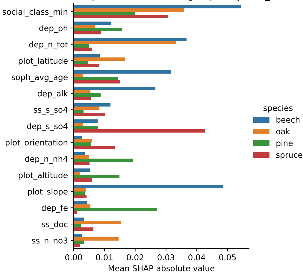
Feature importance for GBDT (grouped by tree_id)
