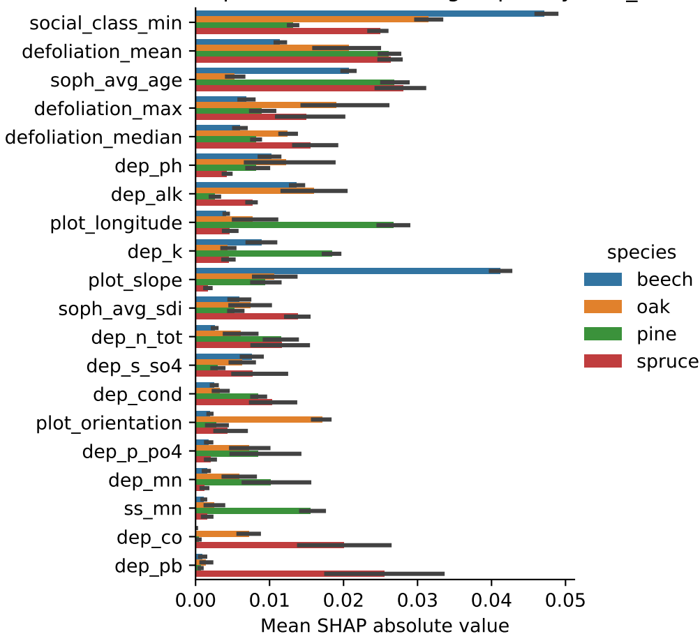
Feature importance for GBDT (grouped by tree_id)
