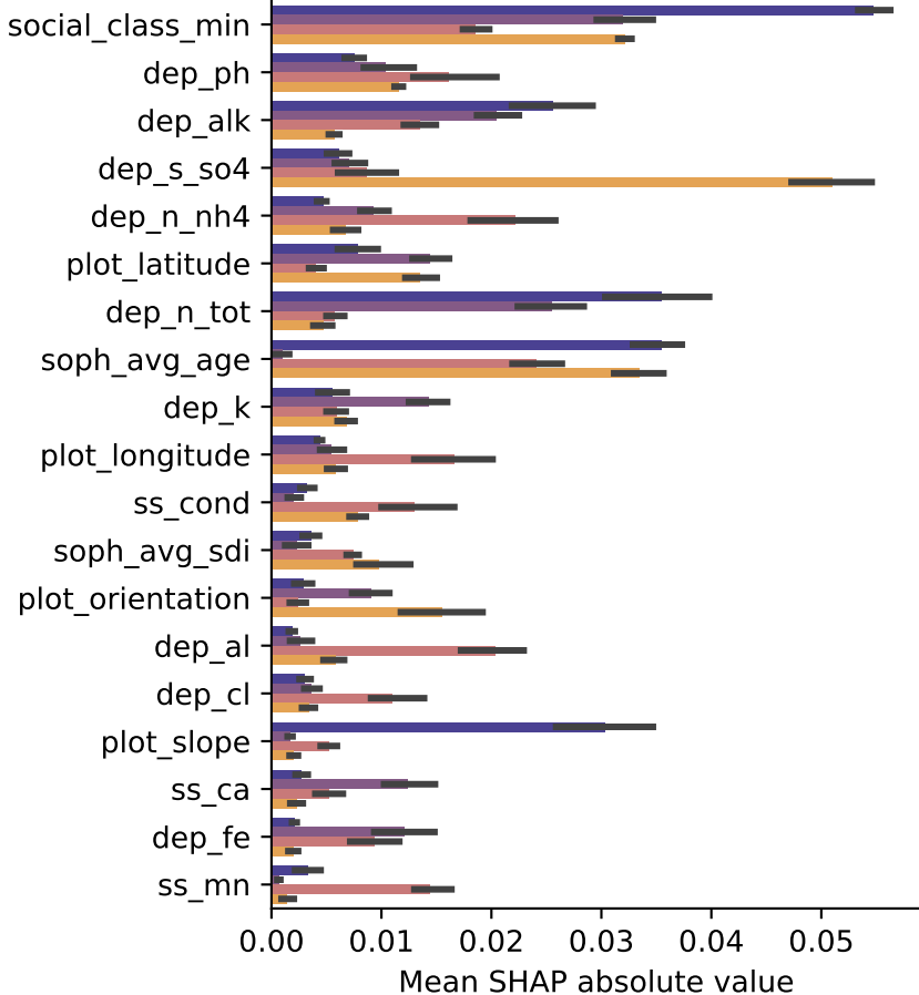
Feature importance for GBDT (grouped by tree_id)
