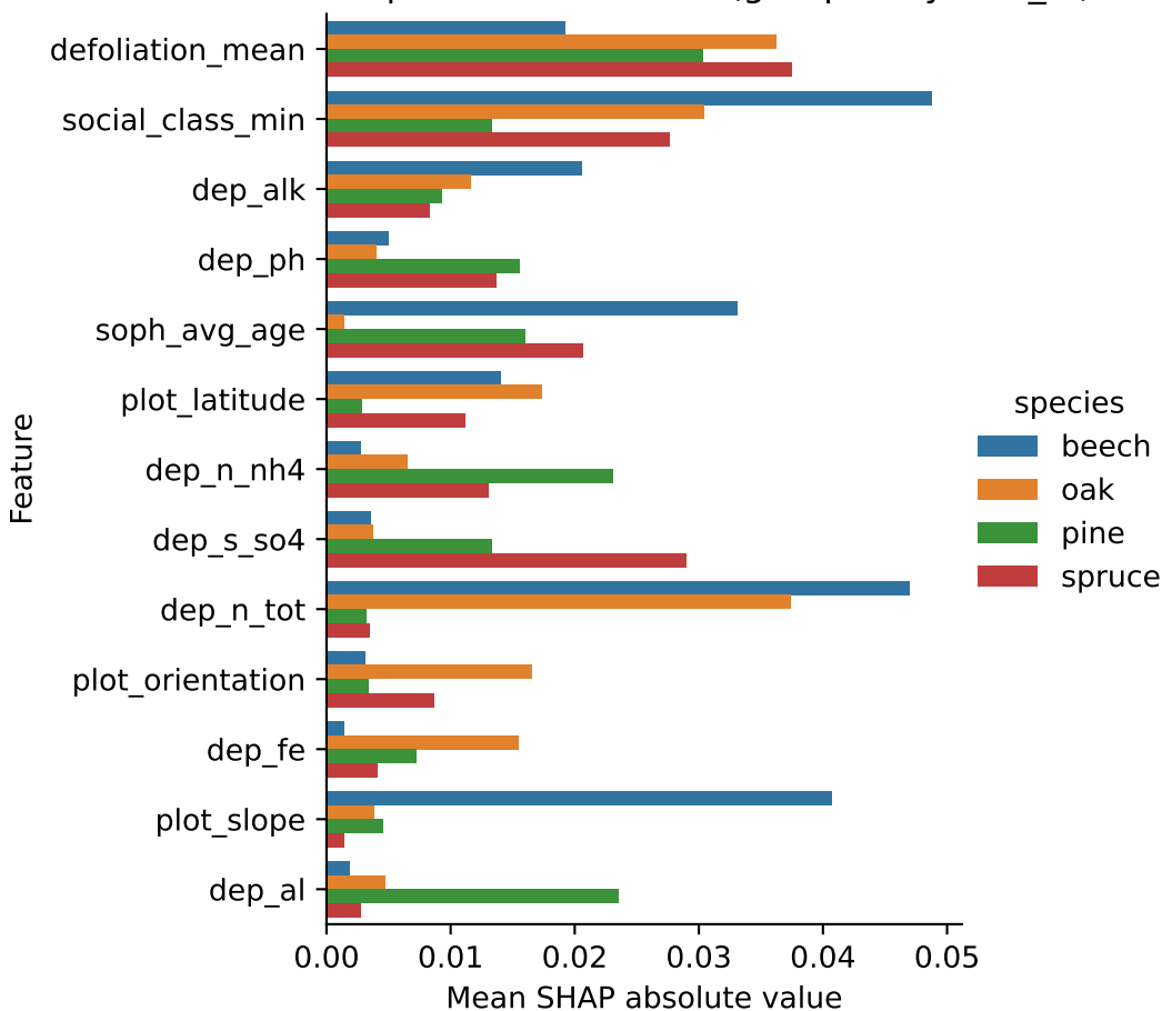
Feature importance for GBDT (grouped by tree_id)
