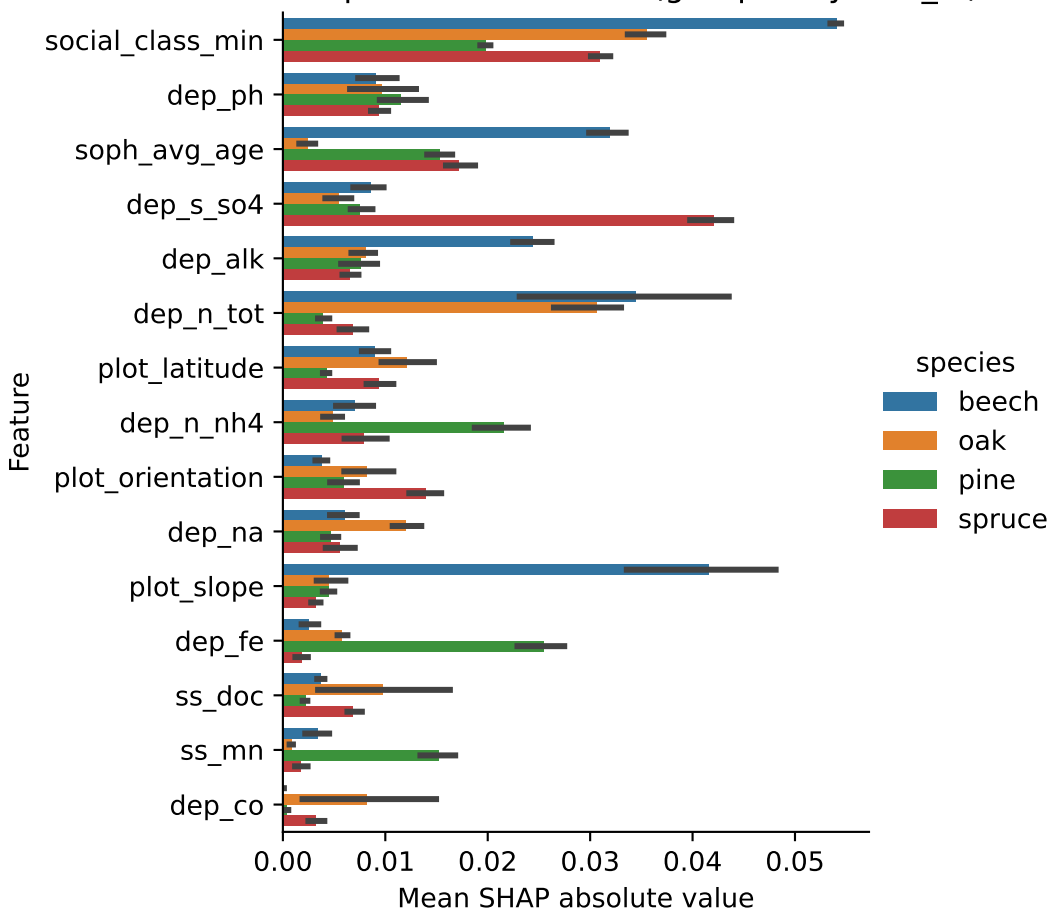
Feature importance for GBDT (grouped by tree_id)
