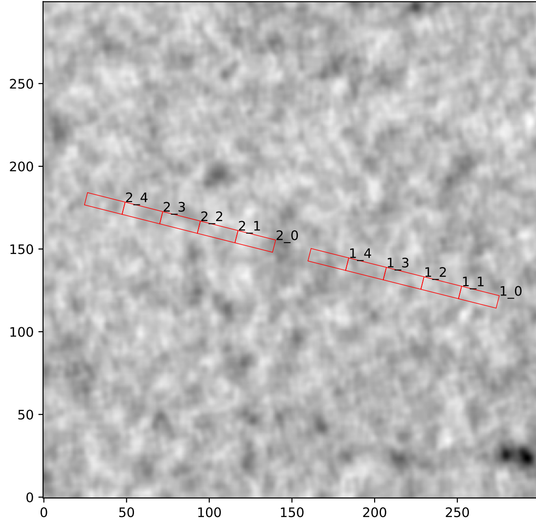
Shards on Sky (DCEID: 96580060)
