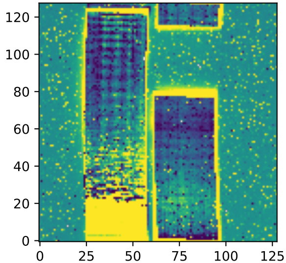
12um Zodi: 32.3 MJy/sr
