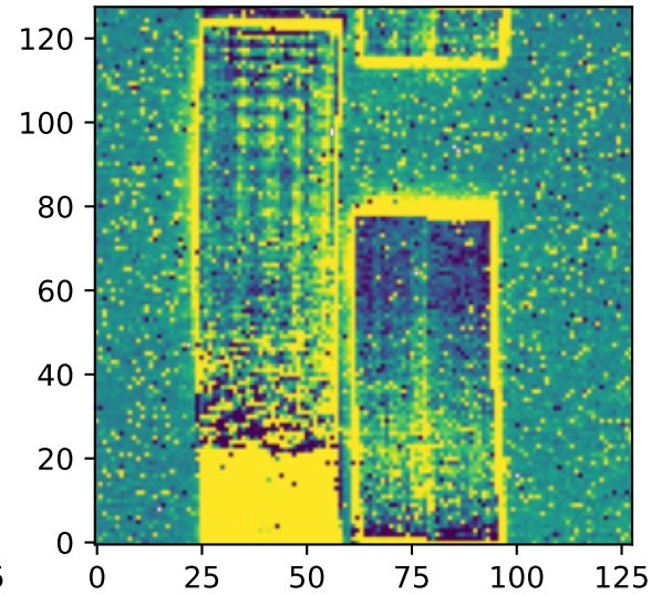
12um Zodi: 40.3 MJy/sr
