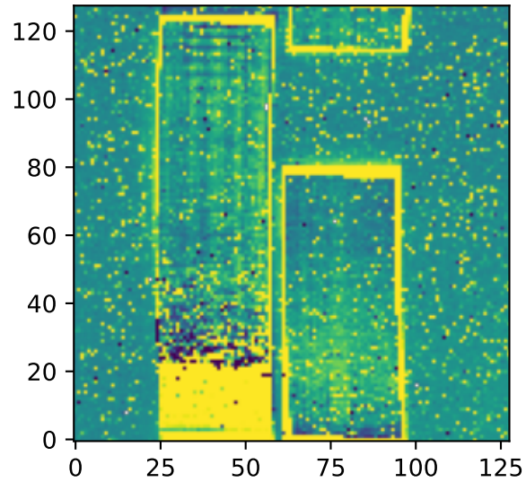
12um Zodi: 23.8 MJy/sr
