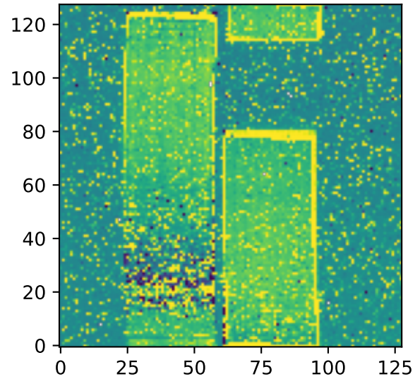
12um Zodi: 13.8 MJy/sr
