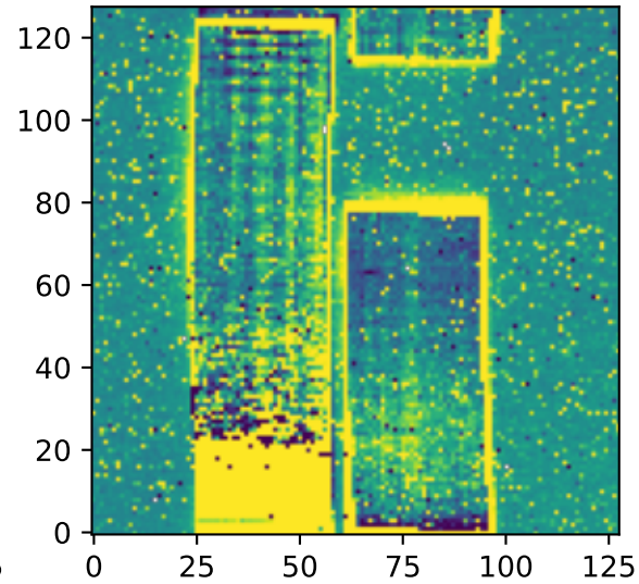
12um Zodi: 31.9 MJy/sr
