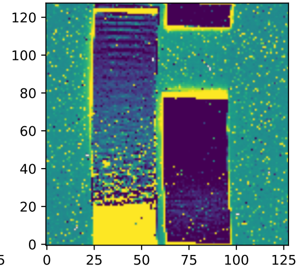
12um Zodi: 39.5 MJy/sr
