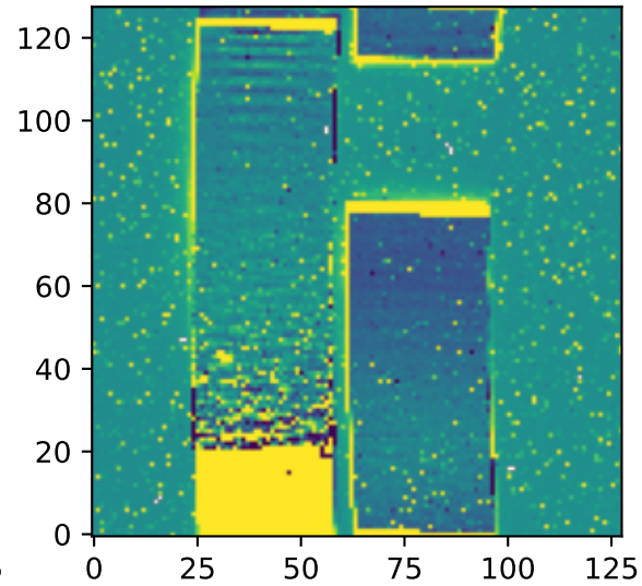
12um Zodi: 23.3 MJy/sr
