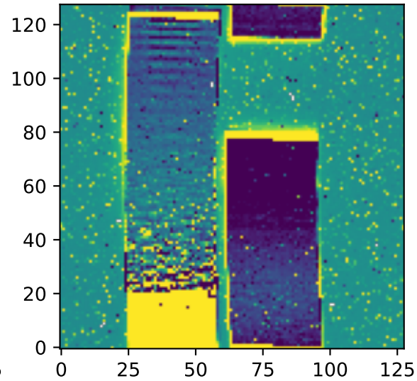
12um Zodi: 30.4 MJy/sr
