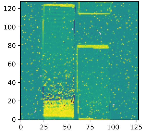
12um Zodi: 14.4 MJy/sr
