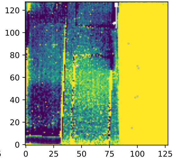
12um Zodi: 39.4 MJy/sr
