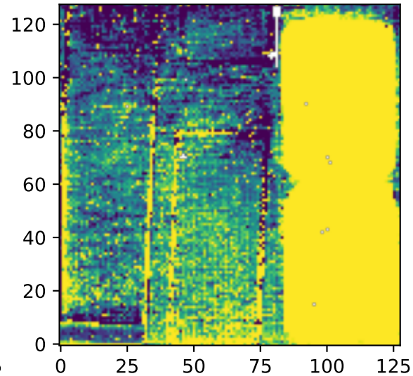
12um Zodi: 32.7 MJy/sr
