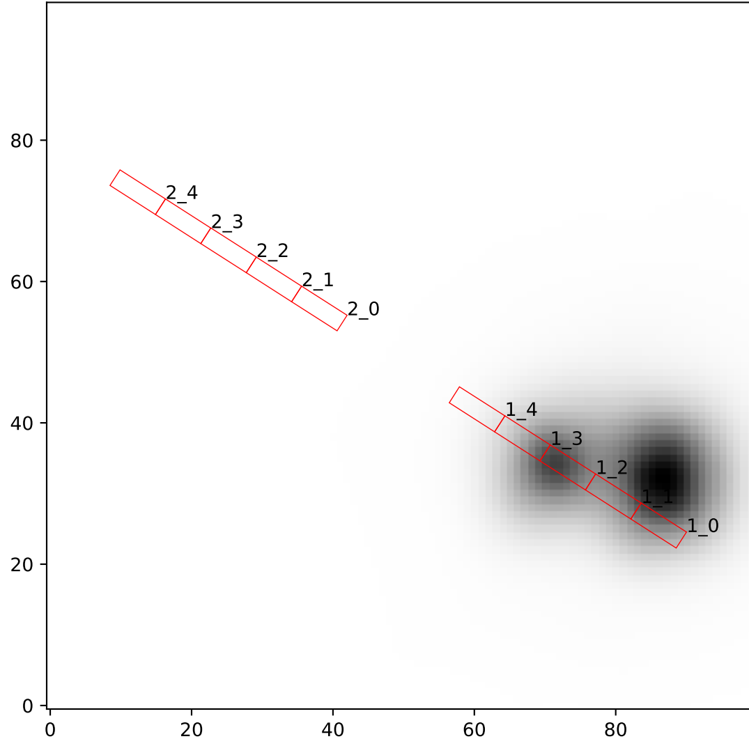
Shards on Sky (DCEID: 13575456)
