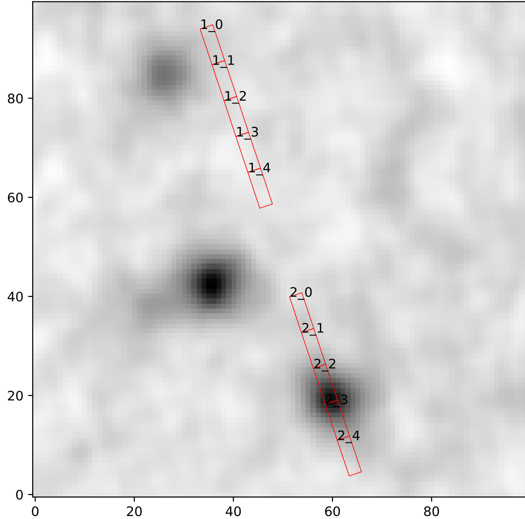
Shards on Sky (DCEID: 68386179)
