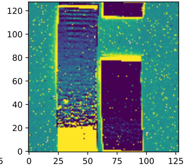
12um Zodi: 40.0 MJy/sr
