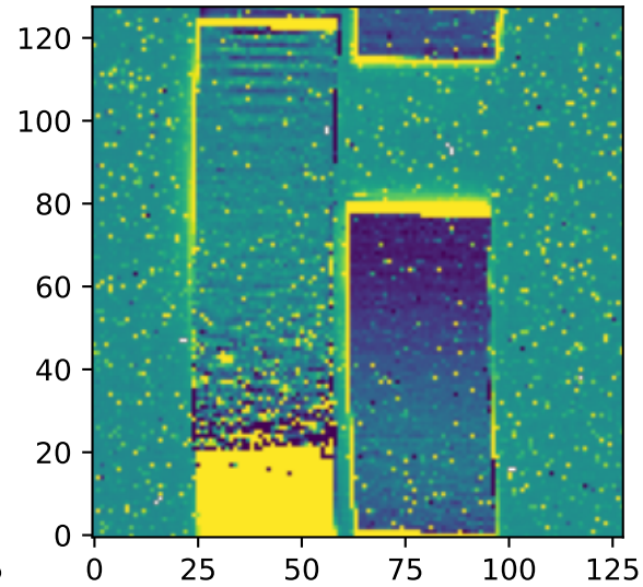
12um Zodi: 31.8 MJy/sr
