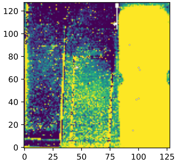
12um Zodi: 42.3 MJy/sr
