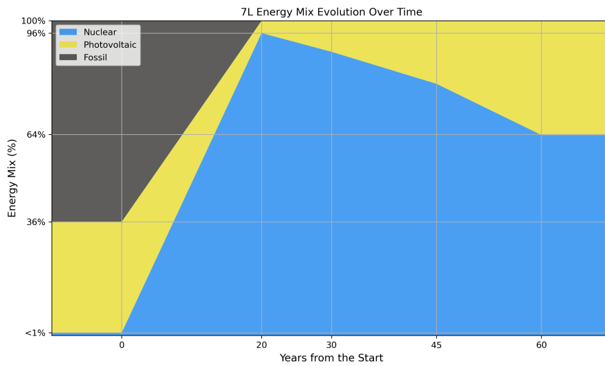
Figure 22: Local energy mix evolution over time.
