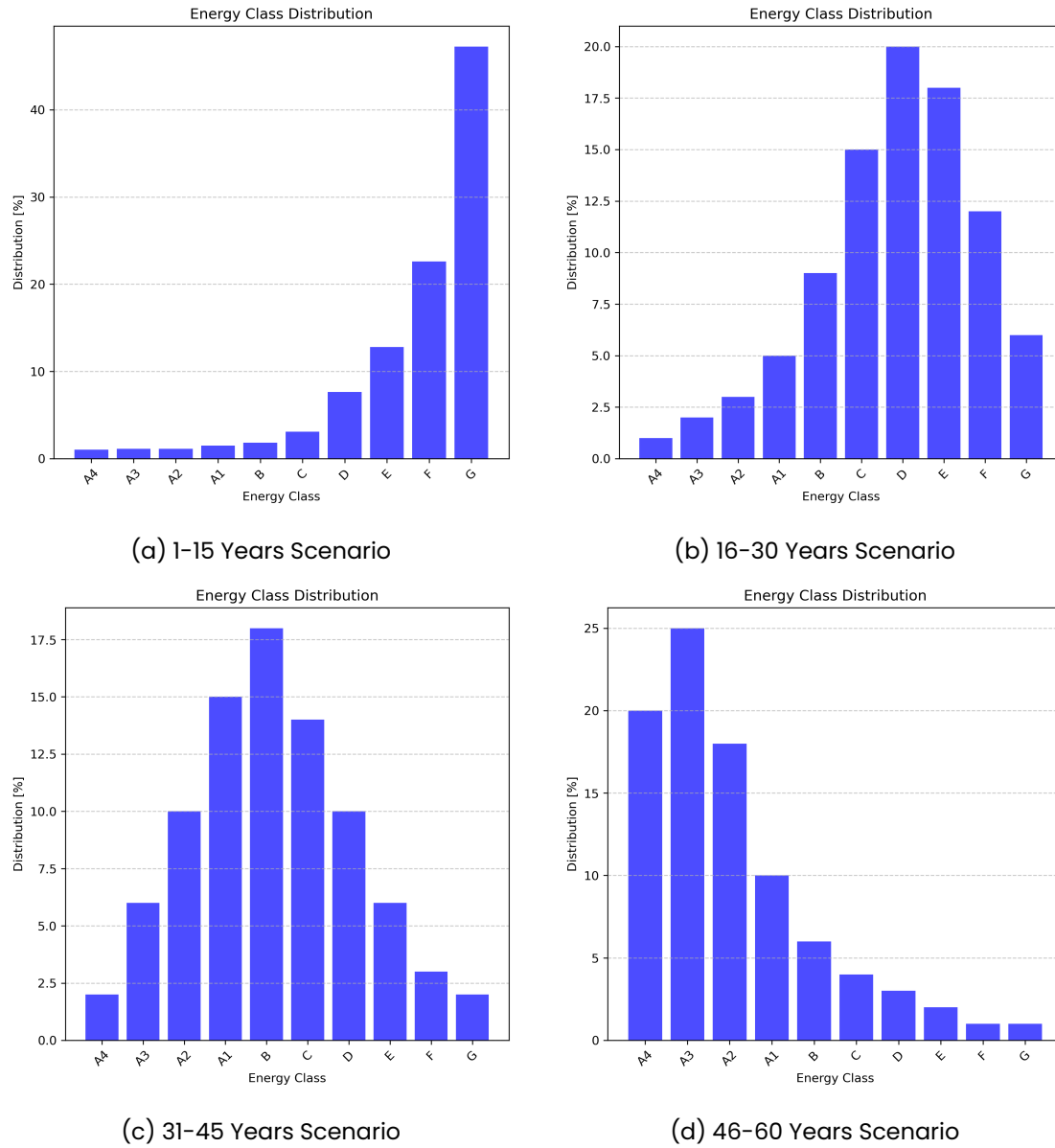
Figure 3: Distribution of energy classes in the residential sector for the four scenarios.
