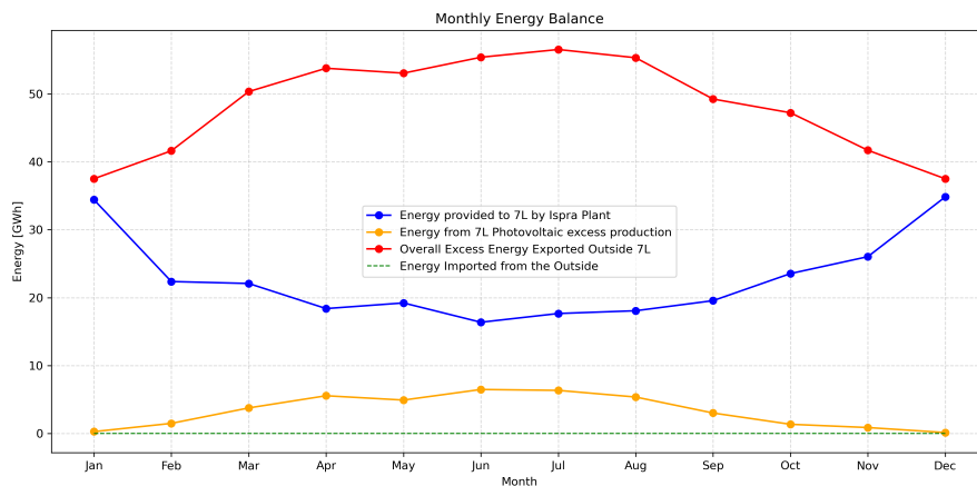
Figure 21: 1-year energy balance for the last simulated period (year 45 to 60).
