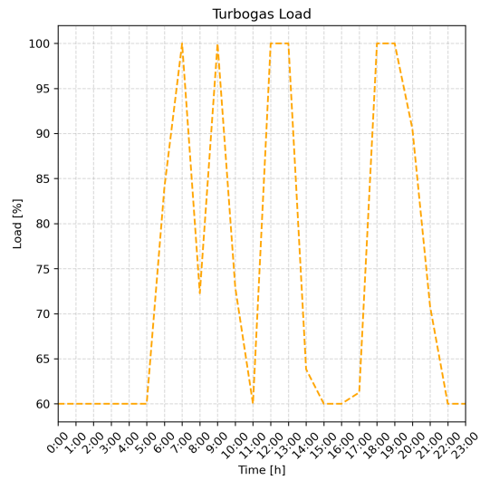
Figure 20: Example of 1-day load profile for gas turbine.
