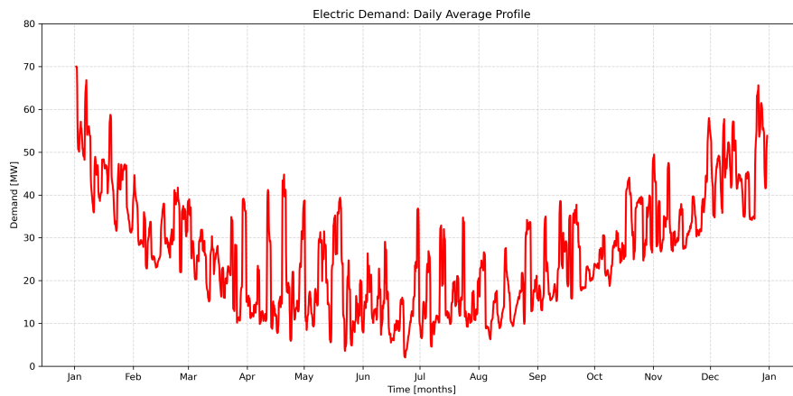
Figure 16: Example of daily average electricity demand profile for the regional grid across a year.
