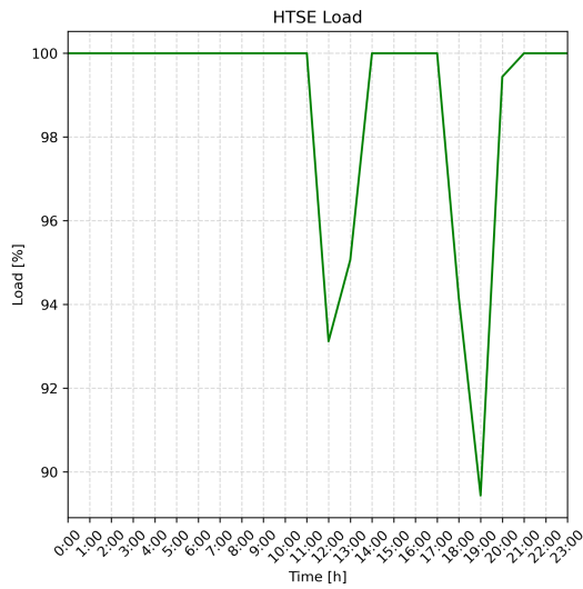
Figure 19: Example of 1-day load profile for HTSE.
