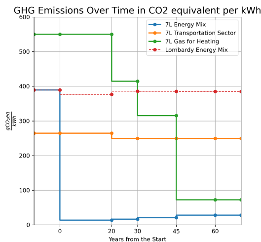
Figure 23: GHG emissions over time.
