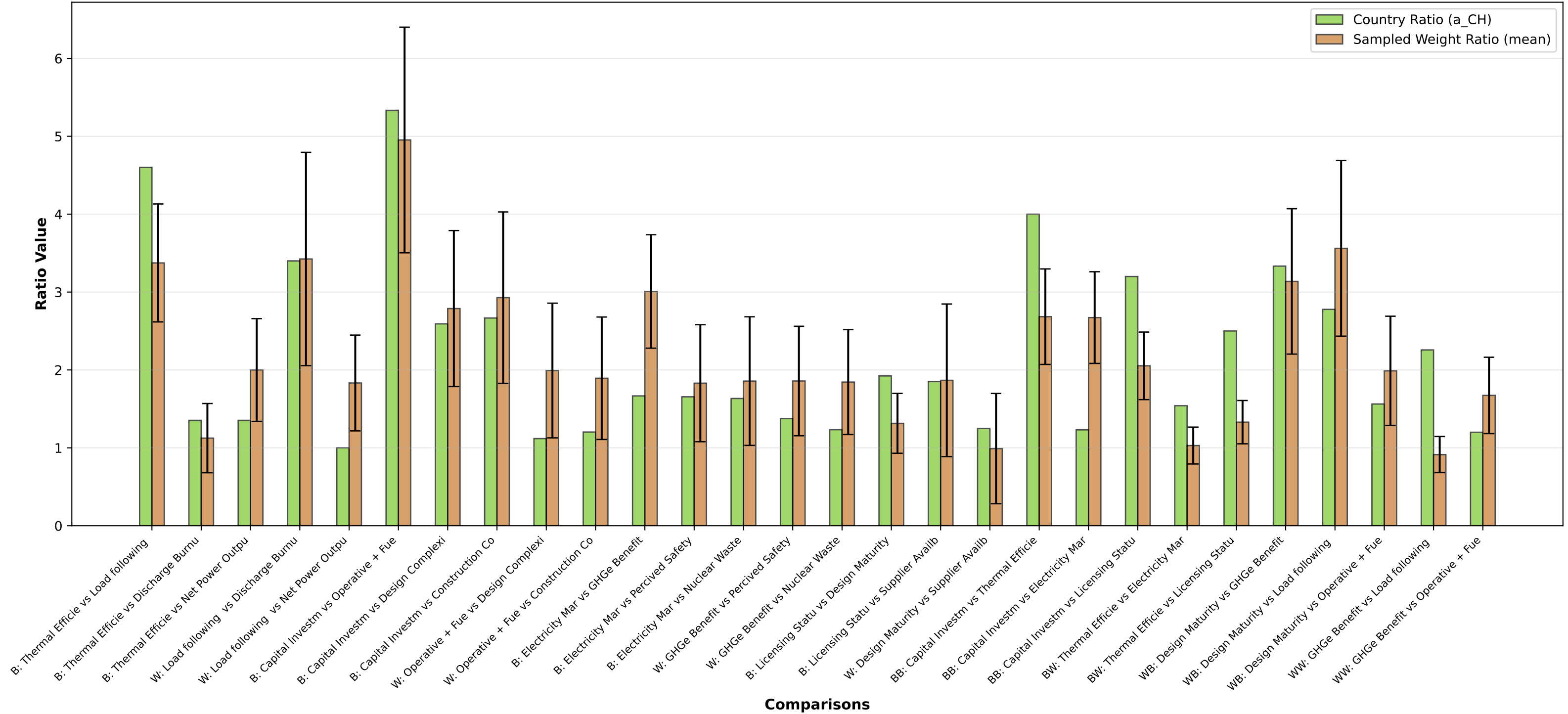
Country vs Sampled Weight Ratios (mean \pm \sigma ) - Elicitation 9 (CH)
