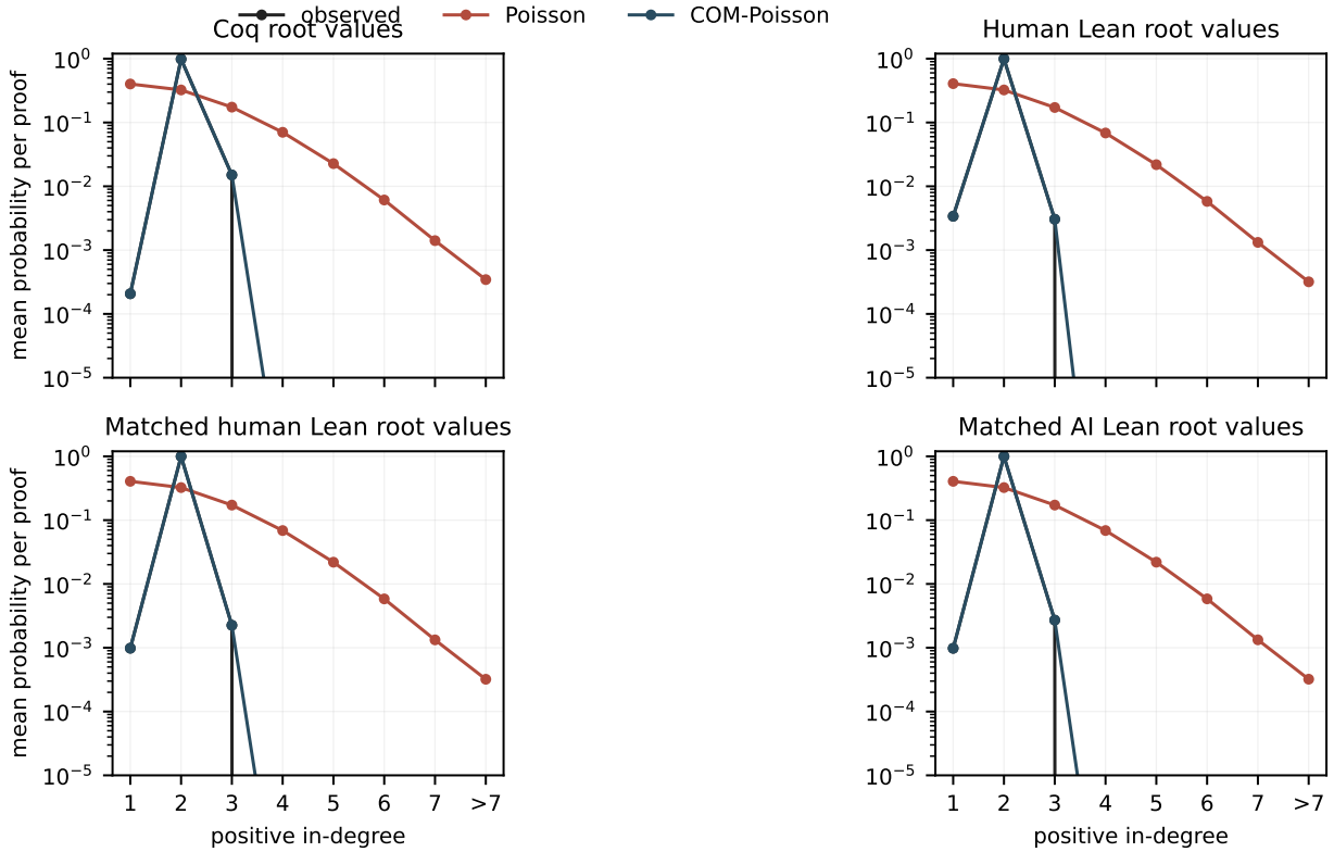
Figure 5: Positive local arity under one constructor schema. Curves average network-level probabilities, giving each proof equal weight; the last category combines degrees above seven. Once application is binary on both sides, Coq and Lean are similarly concentrated at two. The fitted Poisson necessarily places mass on arities absent from the grammar.
