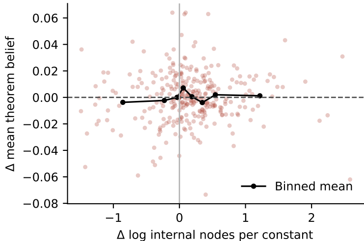
Structural change is epistemically decoupled ( \rho_s = 0.05 )
