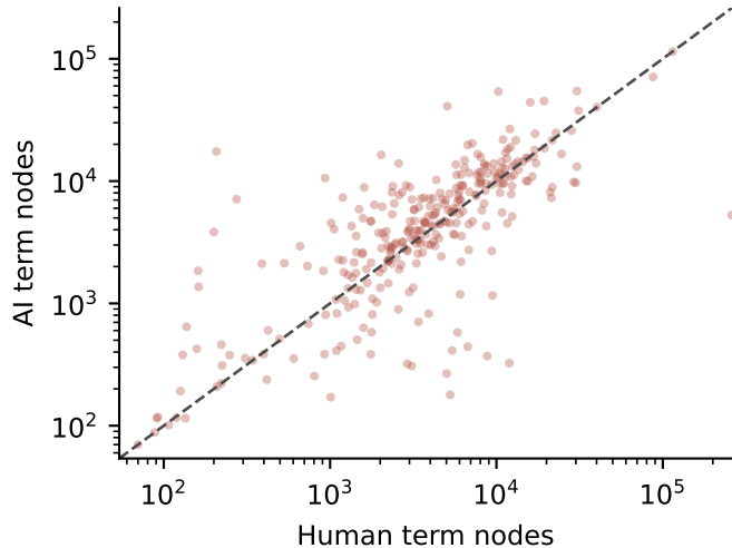
Elaborated terms: \rho_s = 0.76
