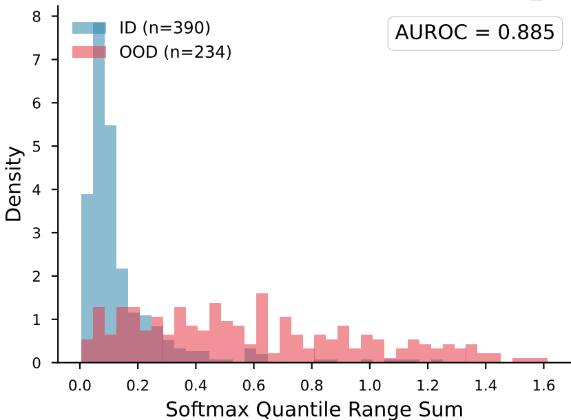
Softmax Quantile Range Sum — ID vs tail_0
