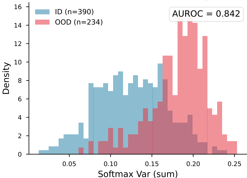
Softmax Var (sum) — ID vs tail_0
