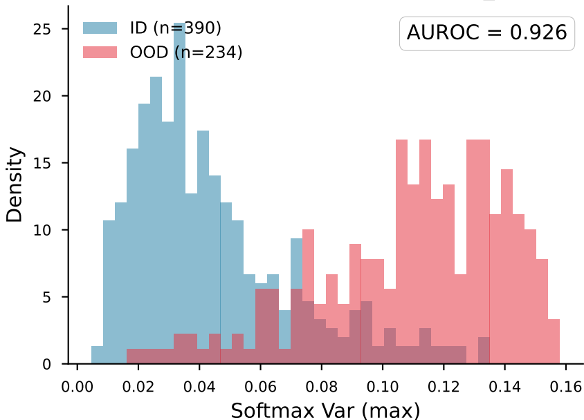
Softmax Var (max) — ID vs tail_0
