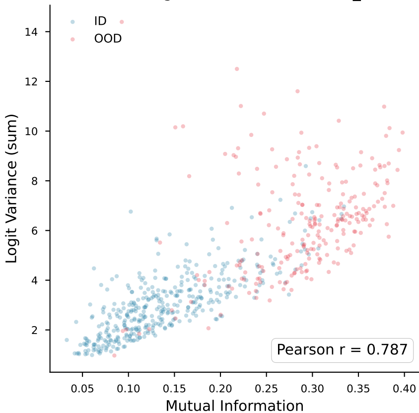
MI vs Logit Variance — ID vs tail_0
