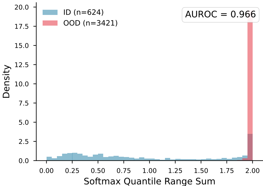
Softmax Quantile Range Sum — ID vs bloodmnist
