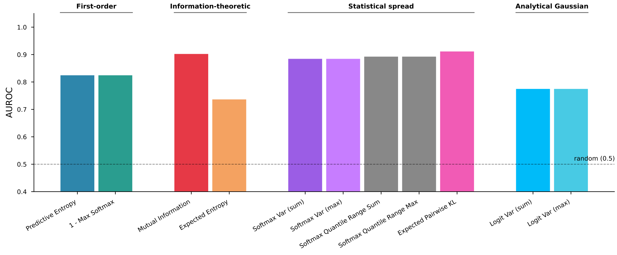
OOD-detection AUROC by score family — ID vs bloodmnist
