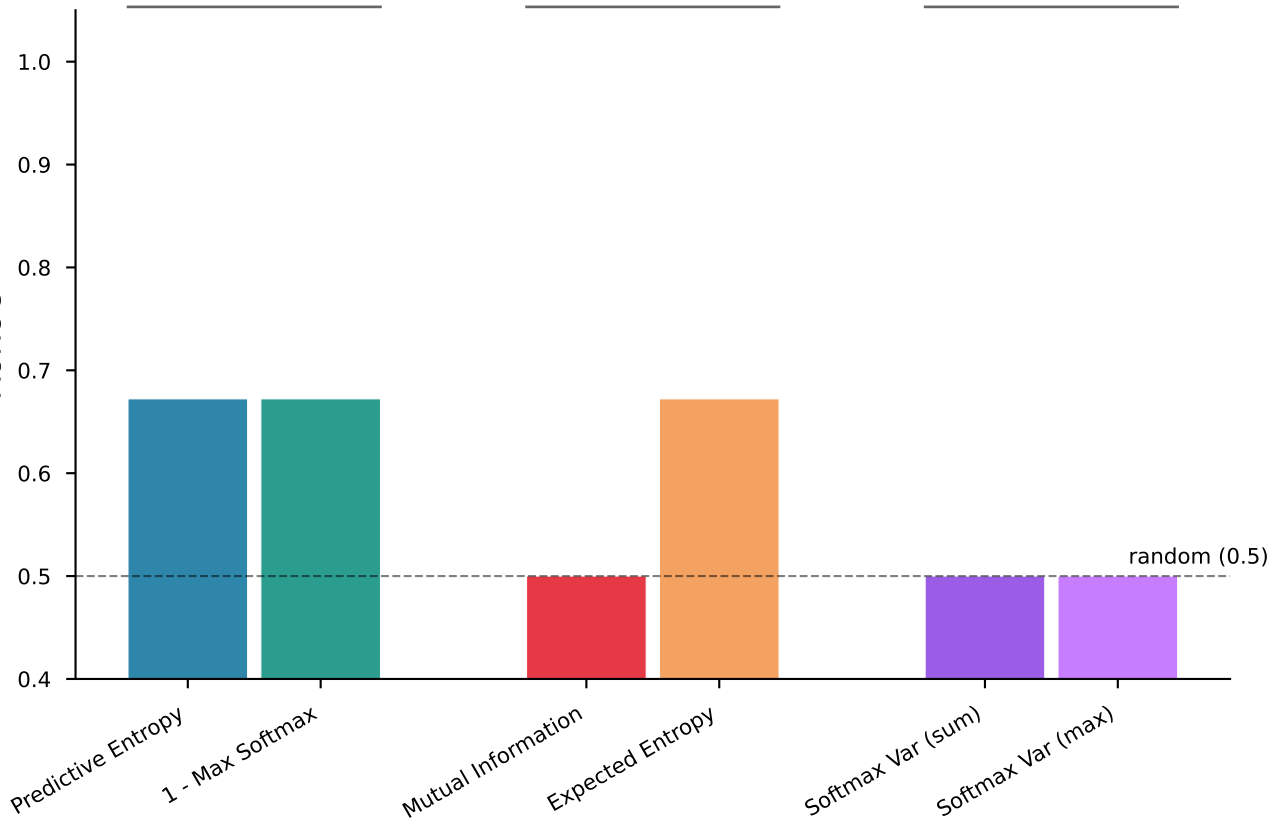
OOD-detection AUROC by score family — ID vs organamnist
