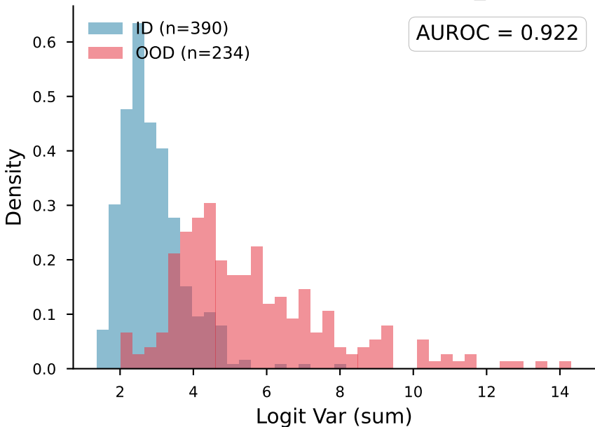
Logit Var (sum) — ID vs tail_0
