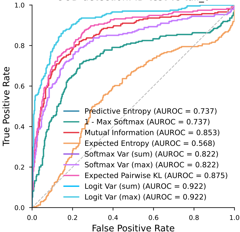
OOD detection: ID test vs tail_0
