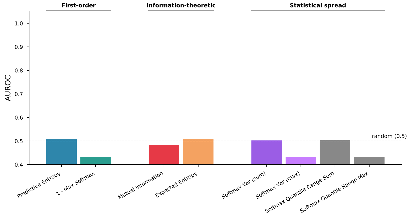
OOD-detection AUROC by score family — ID vs bloodmnist
