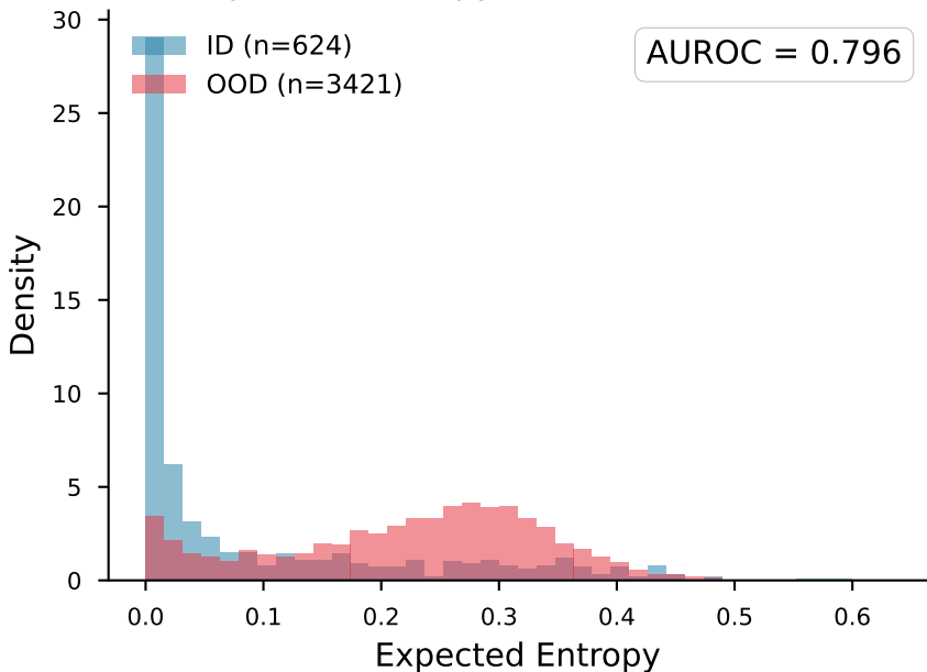
Expected Entropy — ID vs bloodmnist
