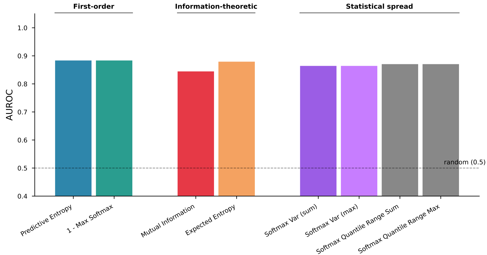
OOD-detection AUROC by score family — ID vs tail_0
