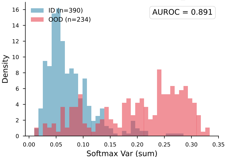
Softmax Var (sum) — ID vs tail_0
