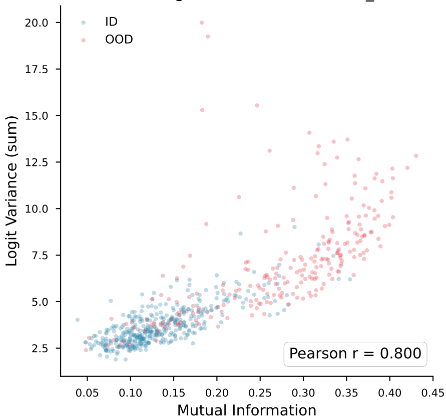
MI vs Logit Variance — ID vs tail_0
