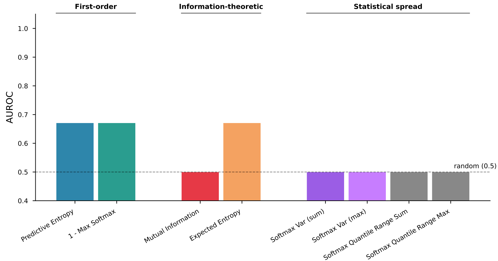
OOD-detection AUROC by score family — ID vs organamnist
