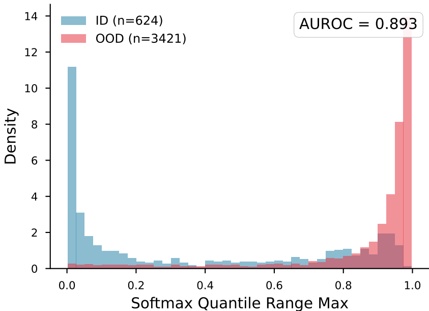
Softmax Quantile Range Max — ID vs bloodmnist
