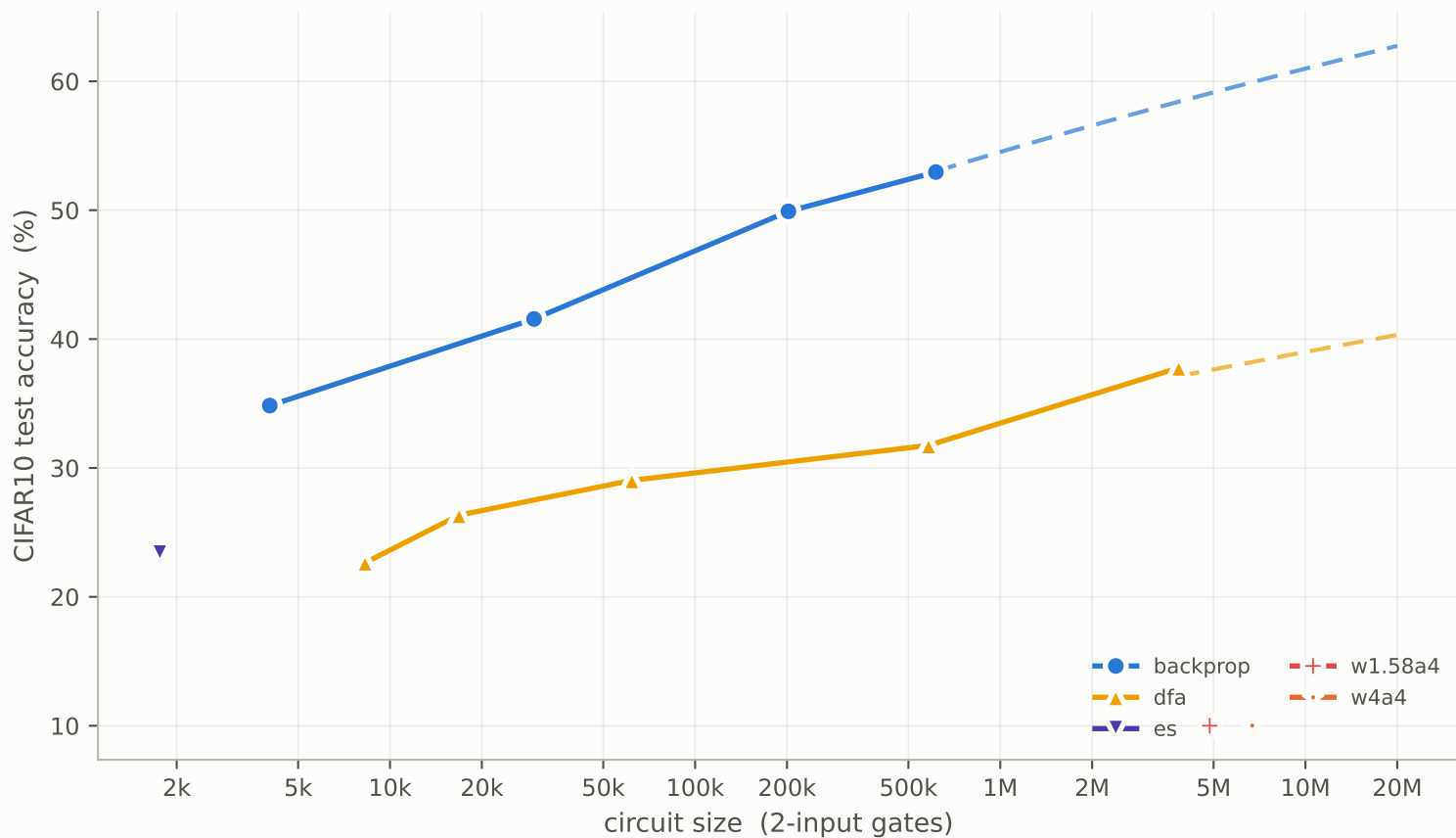
CIFAR10 accuracy vs circuit size
