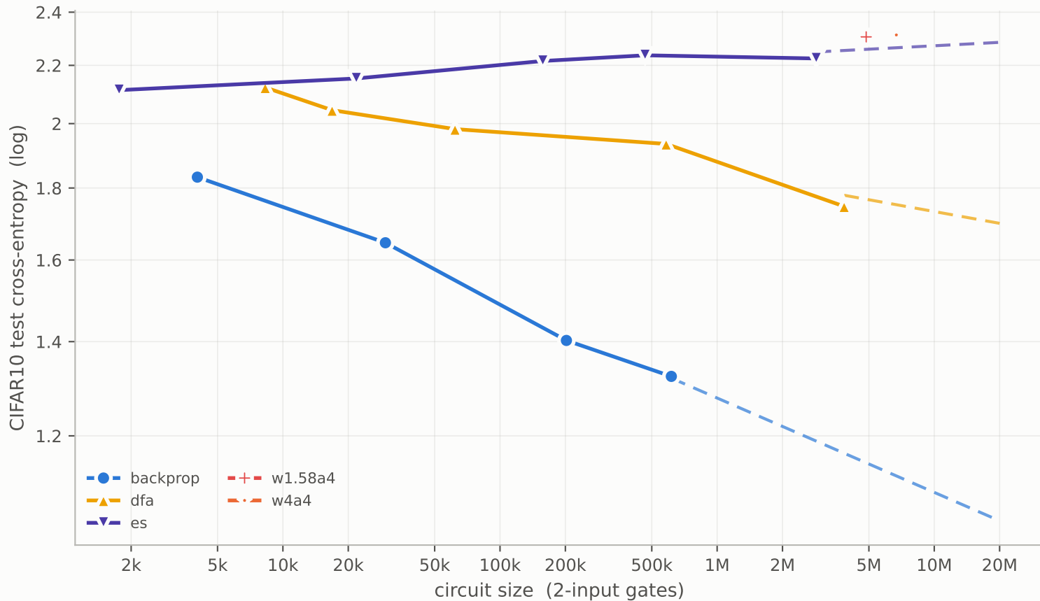
CIFAR10 loss vs circuit size (log-log)
