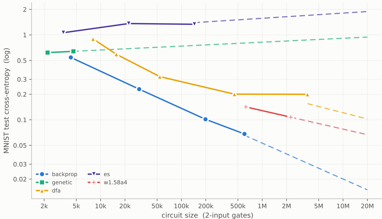
MNIST loss vs circuit size (log-log)
