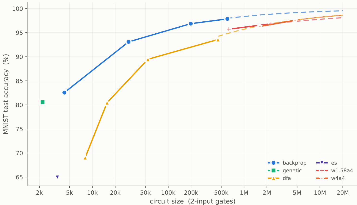
MNIST accuracy vs circuit size
