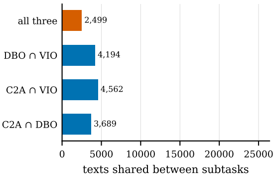
2025: 11,870 distinct texts
