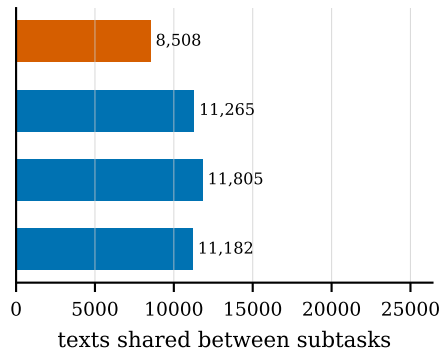
2026: 22,369 distinct texts
