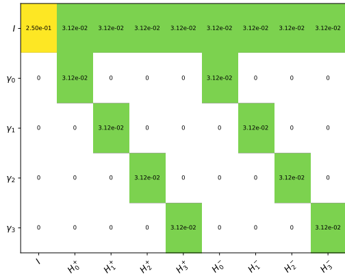
Hopping expansion
